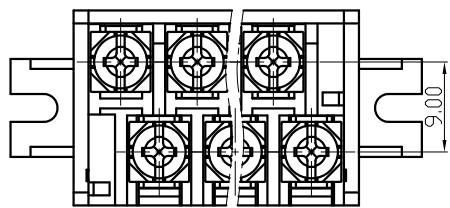
(W/O COVER) A向
